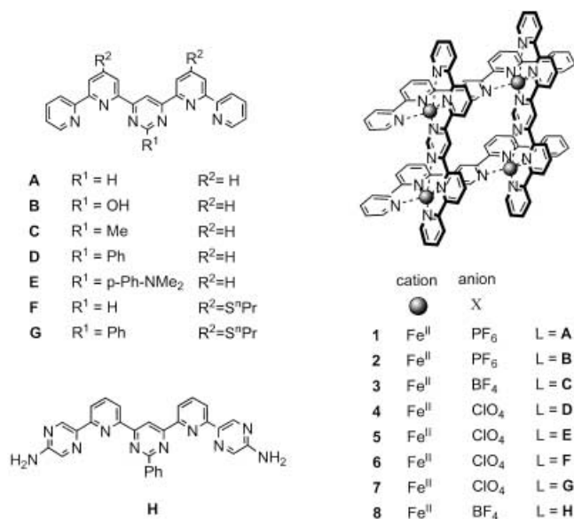
Scheme 1. Ligands A–H and [2 × 2] grid complexes 1–8 .
